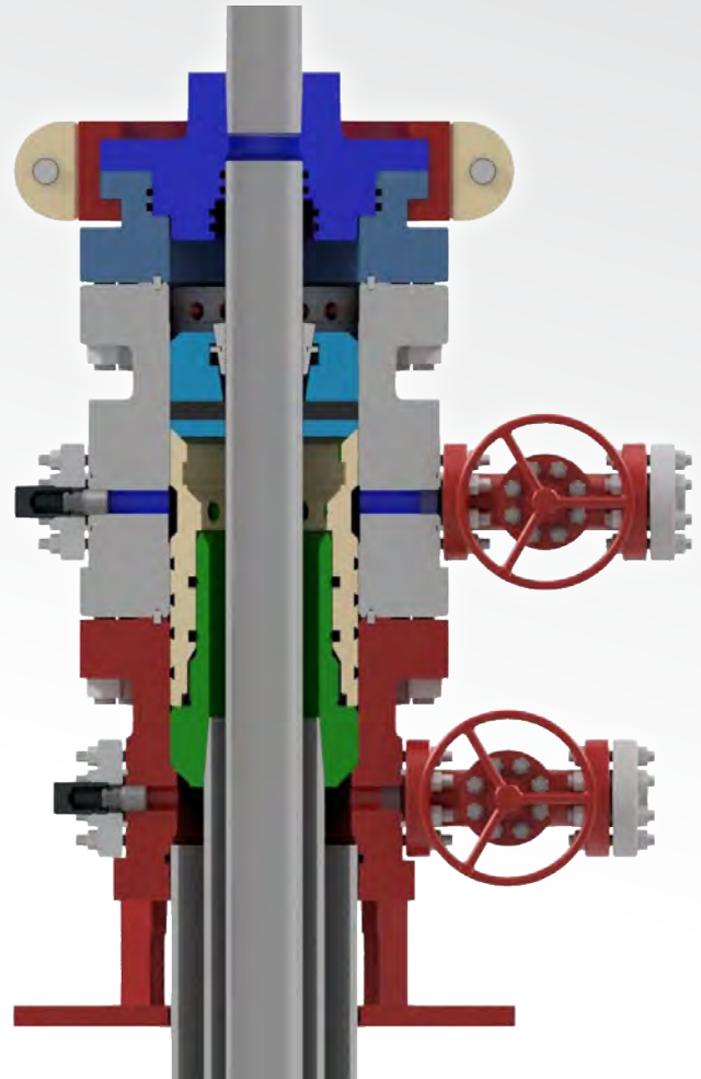
Offline Cementing of Production Casing
