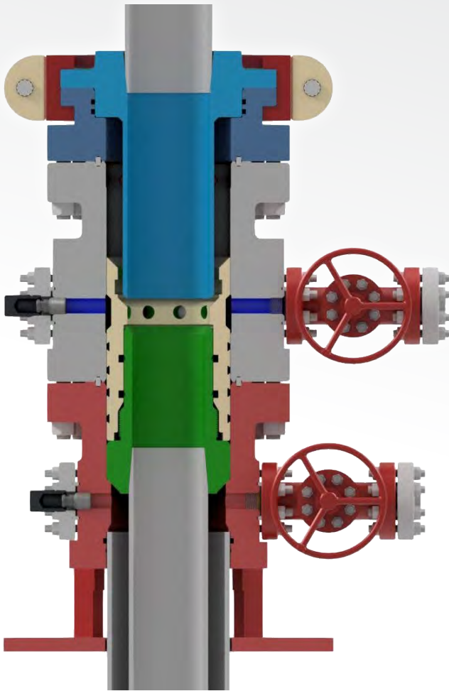
Offline Cementing of Intermediate Casing
